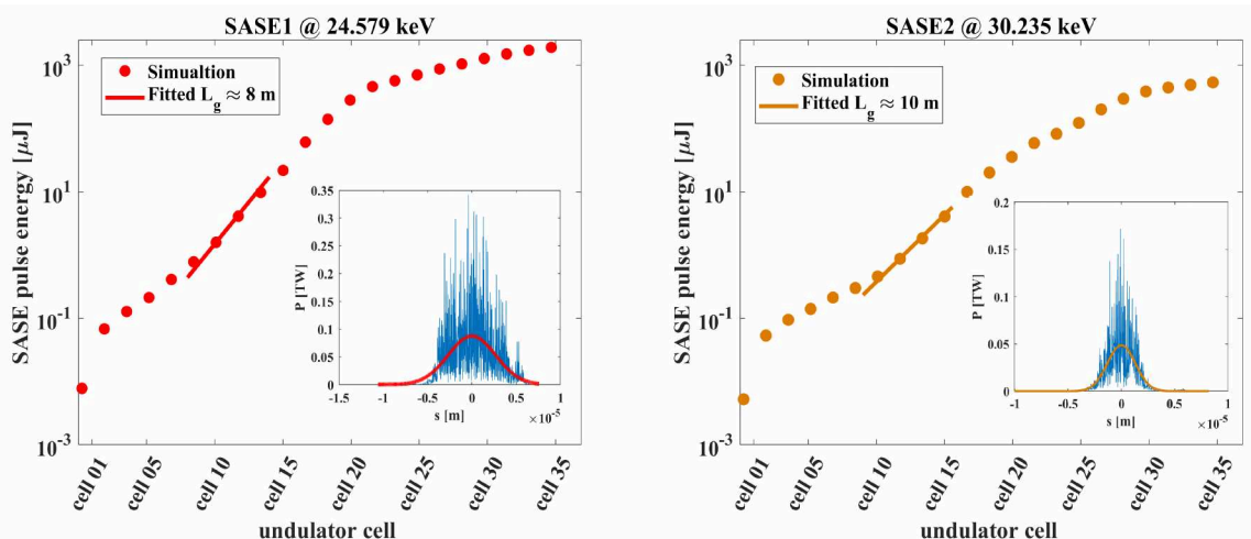
Figure 4: Simulated SASE intensities at 24.58 keV (left) and 30.24 keV (right) for beamlines SASE1 and SASE2, respectively.
