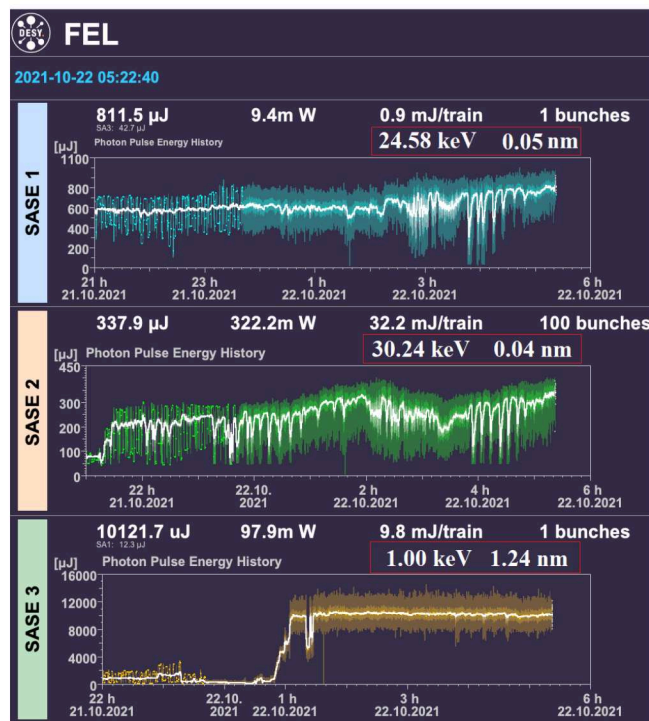
Figure 6: First test run of the EuXFEL delivering hard X-rays of about 0.8 mJ and 0.3 mJ at photon energies of 24 keV and 30 keV for SASE beamlines 1 and 2, respectively, with a simultaneous SASE pulse delivery of about 10 mJ at 1 keV for the SASE beamline 3.
