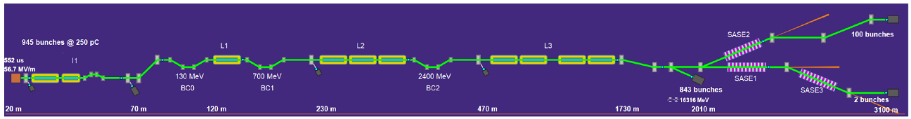
Figure 1: Schematic layout of the European X-ray Free-Electron Laser. I1: injector section; Li: the i-th linear accelerator; BCi: the i-th bunch compressor. SASEi: the i-th undulator beamlines in which SASE1 and SASE2 are hard X-ray lines while SASE3 is a soft X-ray line.
