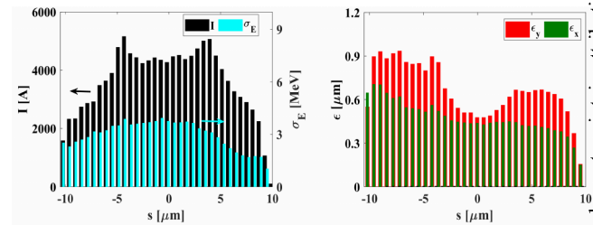
Figure 3: Bunch qualities in front of the undulator beamline SASE1. Left: peak current (left axis) and slice energy spread (right axis); Right: slice horizontal (green) and vertical (red) emittance.
