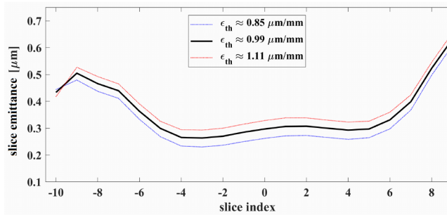
Figure 2: Optimized slice emittance at the injector exit considering different thermal emittance values of the cesium-telluride cathodes as tested at PITZ [19].
