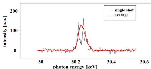
Figure 5: SASE spectrum detected by HIREX [20] for SASE2 with a central photon energy of 30.235 keV.
